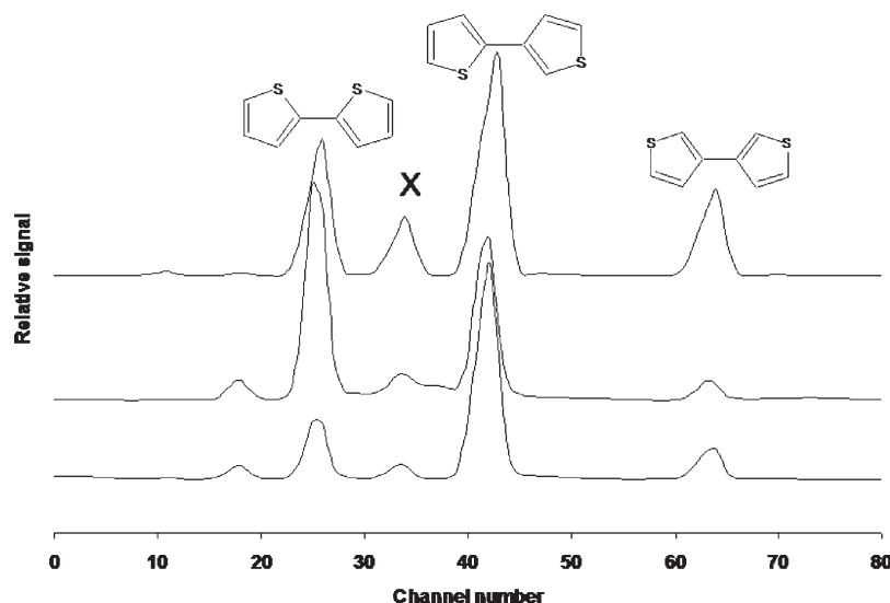
Fig. 5 Partial gas chromatogram of the products of IR LPHP of thiophene (top trace), 2-bromothiophene (middle trace) and 3-bromothiophene (bottom trace), indicating relative yields of 2,2-bithiophene, 2,3-bithiophene and 3,3-bithiophene. The peak marked X arises from one isomer of phenylthiophene, the second isomer being obscured.
